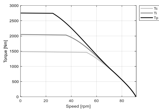
VE - WATER COOLING
