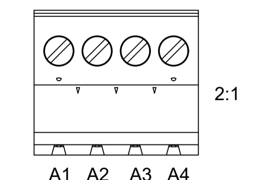
300V Phoenix type Connector
