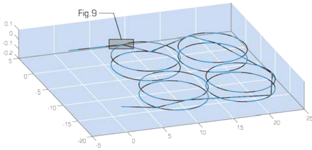
Fig.8 Transition done with G-code line (Black trajectory: Theoretical, Blue trajectory: Tool point).
