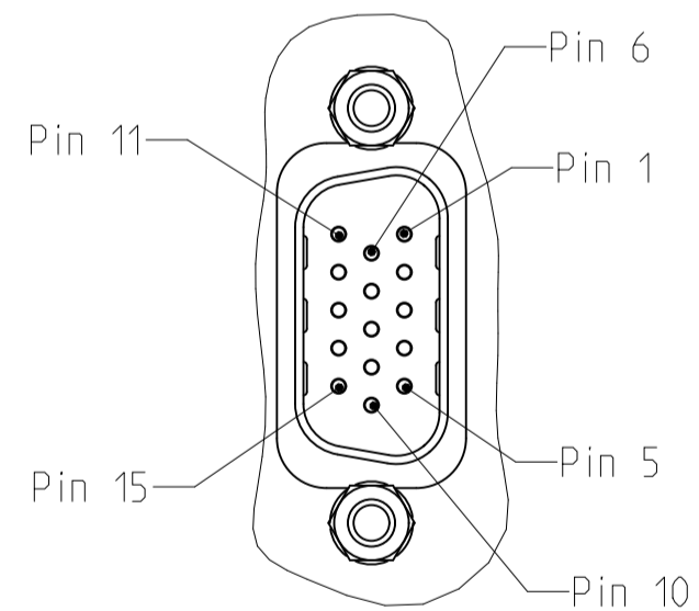
Encoder Connection
